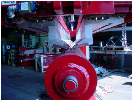
End view of mandrel arm
