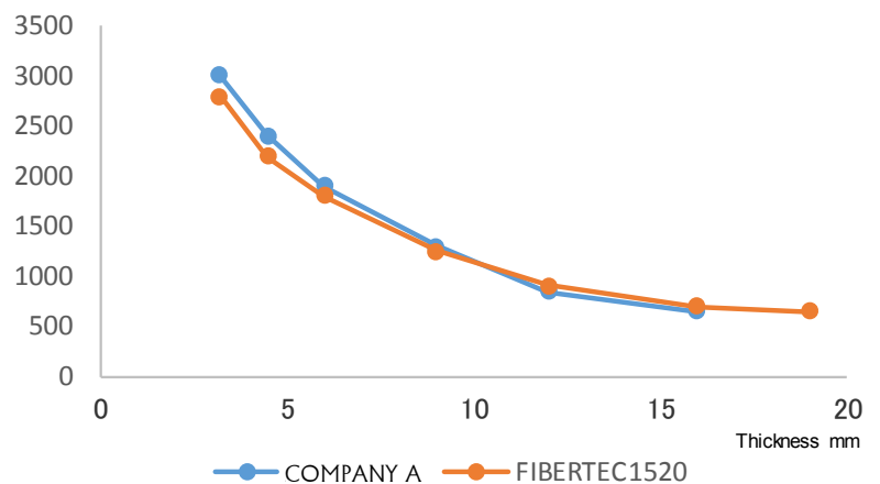
Mild Steel Oxygen Cutting Speed Comparison
